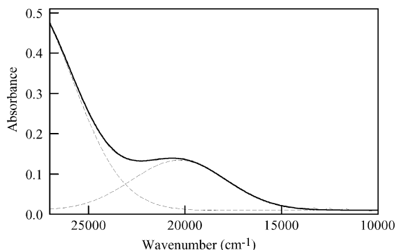
Figure 3. Gaussian deconvolution of the visible bands of the mixed-valent complex [(Ph 2 bpy)(CO) 3 Re I (μ-PCA)Ru III (NH 3 ) 5 ] 4+ ( 4 ; approx. 3 \times 10^{-5} M) obtained by Br 2 oxidation (in CH 3 CN) of the dinuclear complex 3 .
