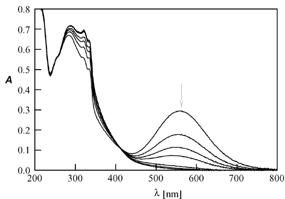
Figure 4. Controlled potential electrolysis of a CH 3 CN solution of [(Ph 2 bpy)(CO) 3 Re I (μ-PCA)Ru II (NH 3 ) 5 ] 3+ ( 3 ; approx. 2 \times 10^{-5} M) at 800 mV in an OTTE cell. The arrow indicates increasing times: t = 0, 1, 2, 3, 4, 8 , and 10 min.
